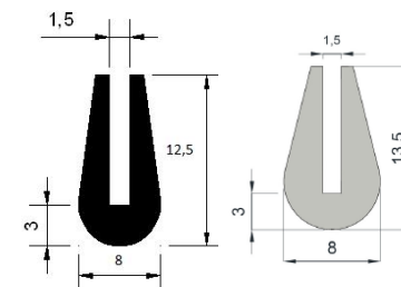
Ref: 05 goma y silicona
